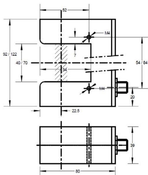
UBA-AT-40/70-24-CU
