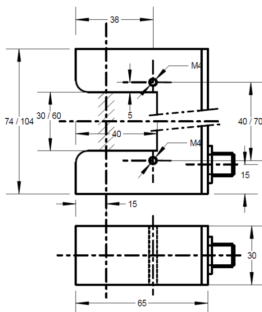
UBA-AT-30/60-24-CU
